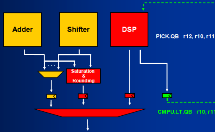
Figure 7: Result forwarding to the next instruction without a delay is possible for useful DSP sequences. .
