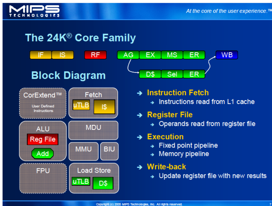
Figure 2: The 24K core family features an eight-stage pipeline divided into four sections
