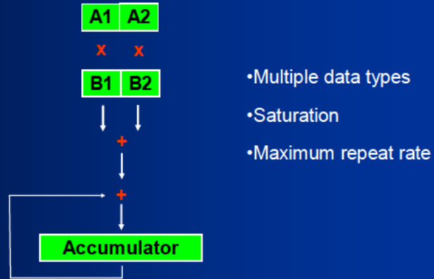
Figure 8: The dot-product-accumulate instruction performs two multiplications and two additions.
