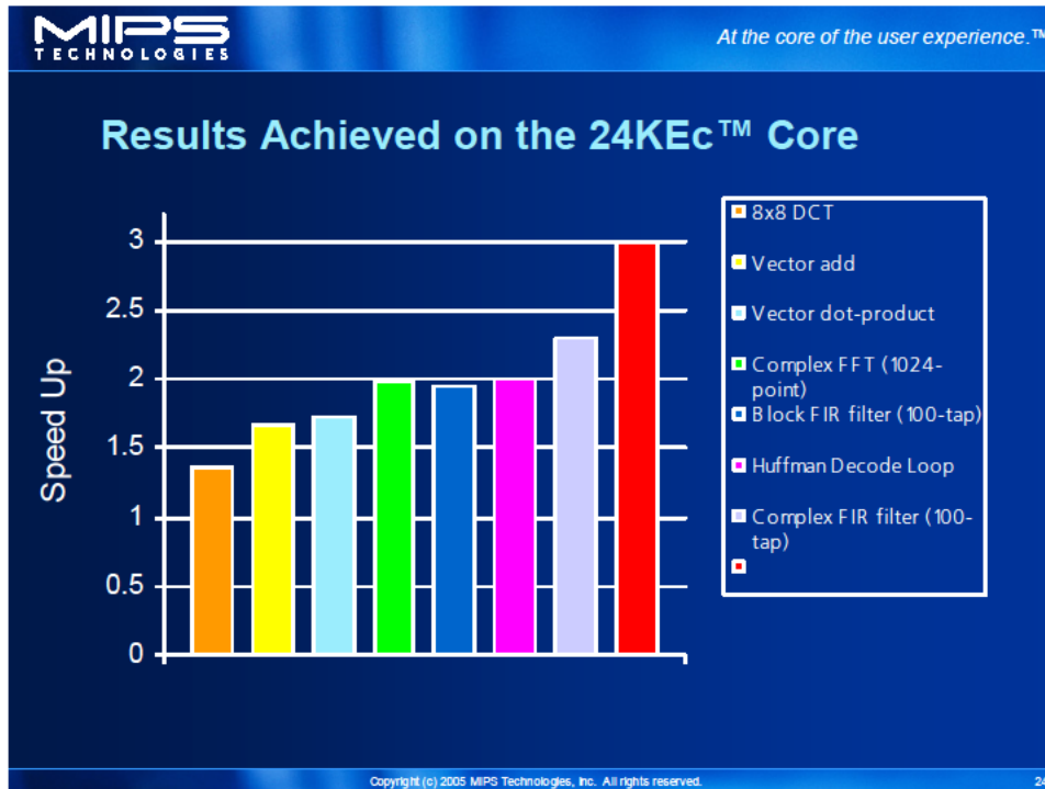
Figure 12: The 24KEc core achieves DSP function code speedups of up to three times the performance of the 24Kc core.
