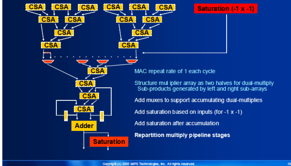
Figure 10: Minimal additional logic was added to support DSP multiply instructions..
