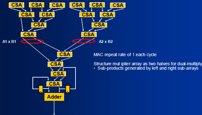
Figure 9: The multiplier data path supports dual-multiply operations and a repeat rate of one MAC per cycle.
