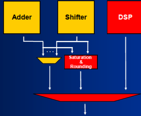
Figure 4: The execution stage data path has critical timing in 24KEc core.
