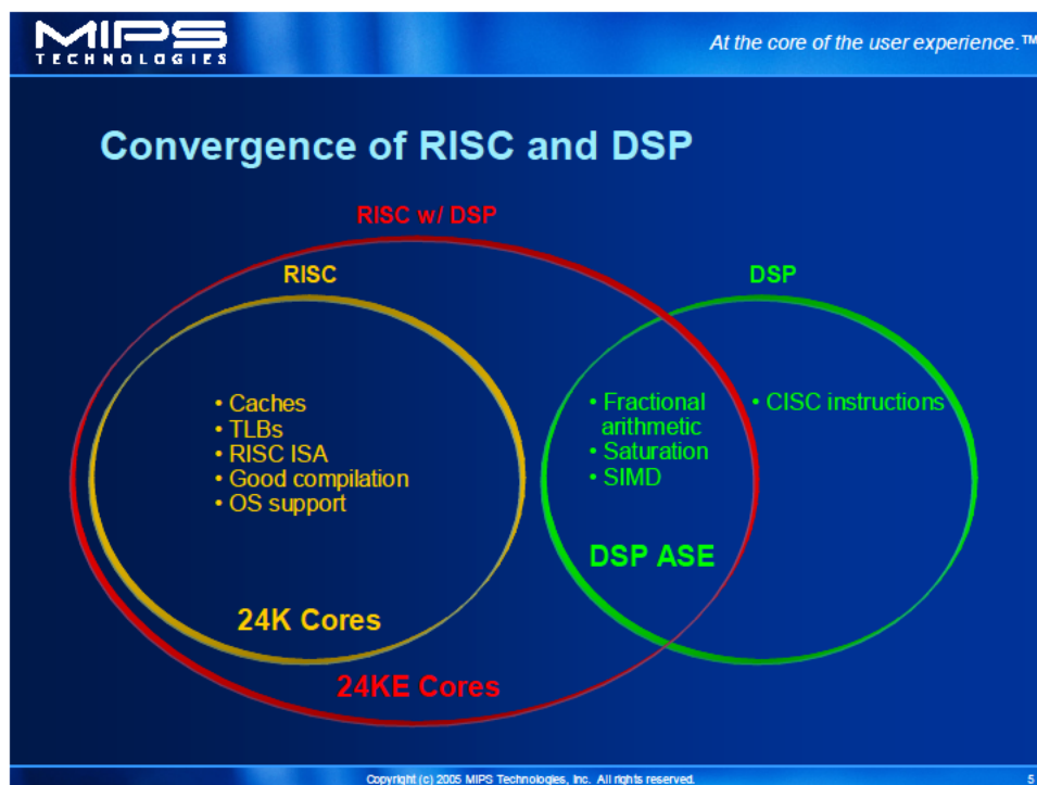
Figure 1: Features of RISC processors and DSPs are converging.
