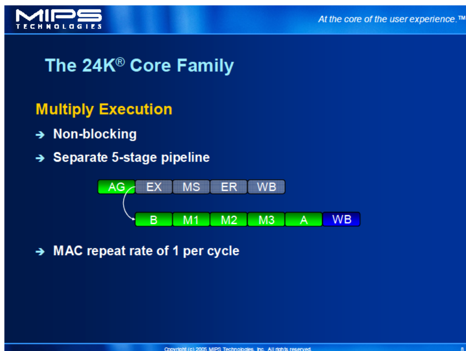
Figure 3: The 24K core family features non-blocking multiply instructions and a repeat rate of one multiply-accumulate instruction per cycle.
