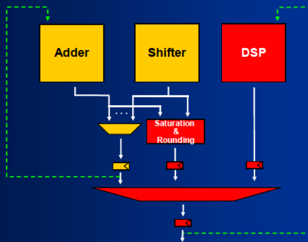
Figure 5: A second cycle is used to forward GPR result of DSP instructions.
